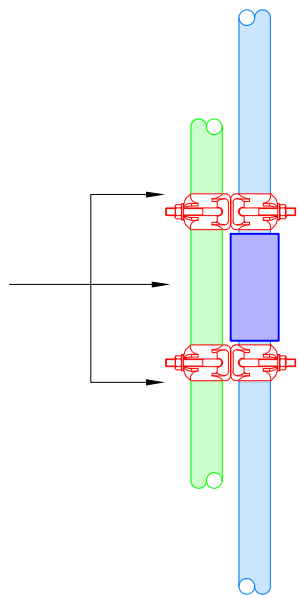
SPLICE CONNECTION DETAIL NTS
